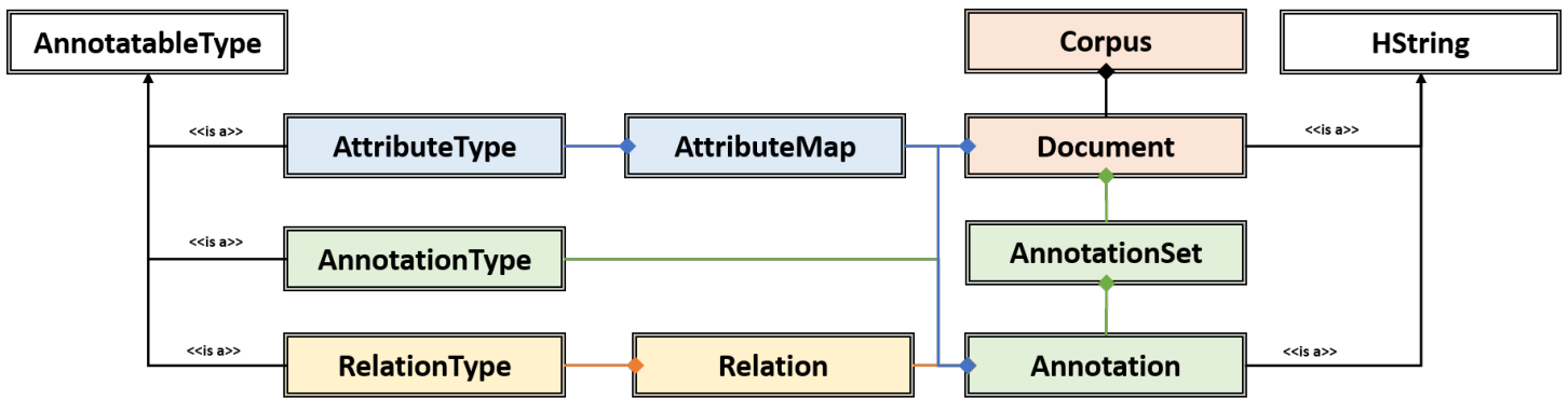
Figure 1. Diagram of Hermes's Core Class
